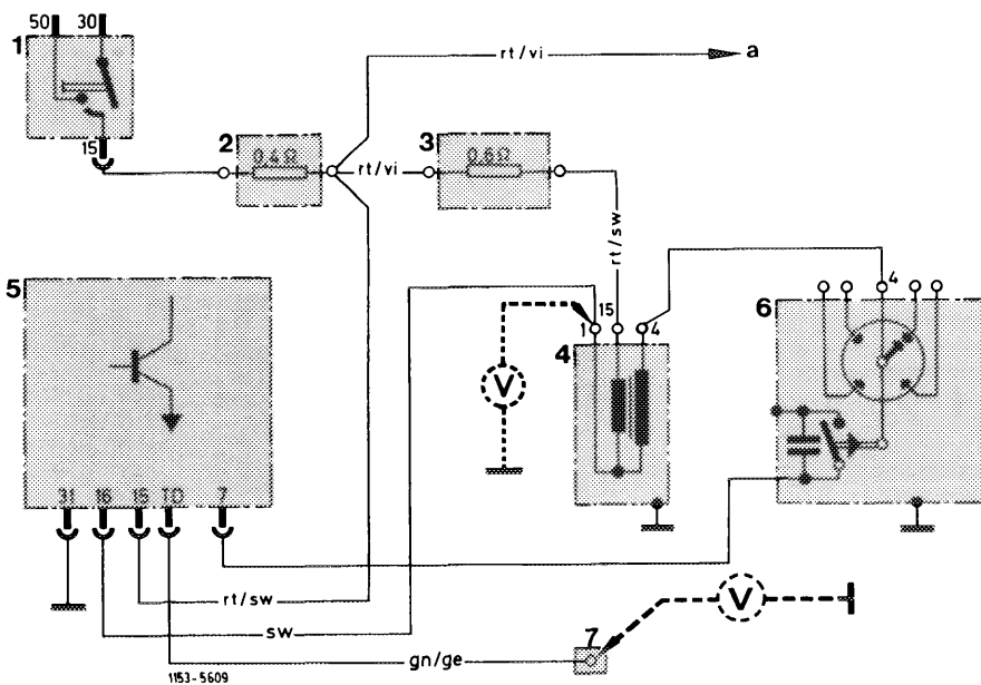
Wiring diagram for SI transistorized coil ignition system with standard switching unit
