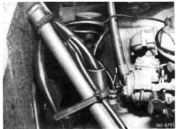
Vacuum connection on engine 130.923
