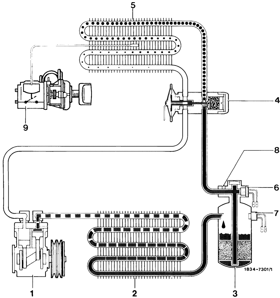
Layout of refrigerant circuit
