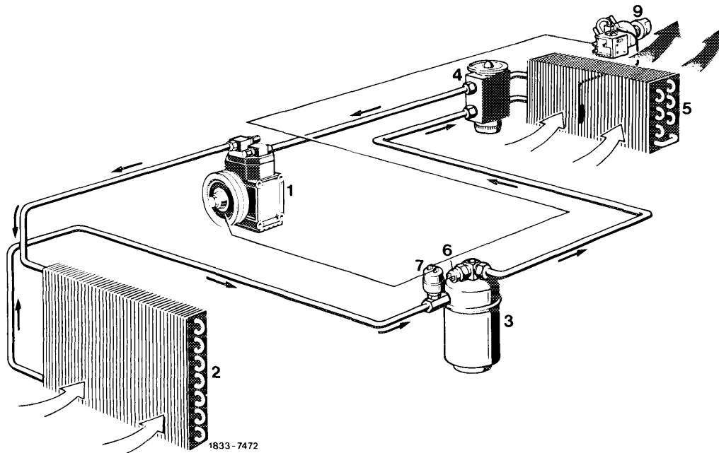
Diagrammatic view of an air-conditioning system
