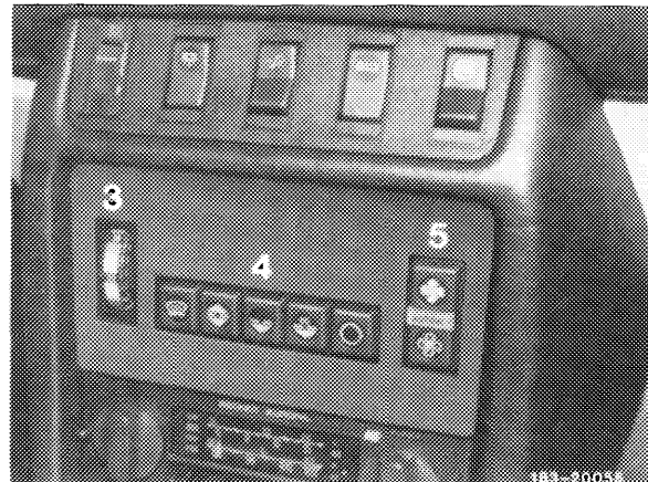
3 Temperature dial 4 Pushbutton switching unit 5 Blower switch
