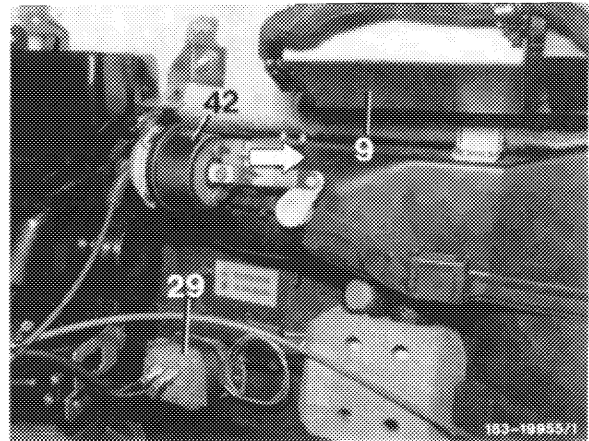
Main air flap closed (arrow), no fresh air supply
