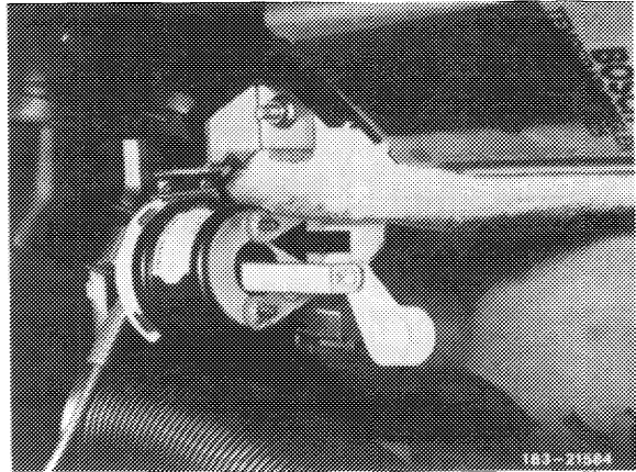
Main air flap opened (arrow)
