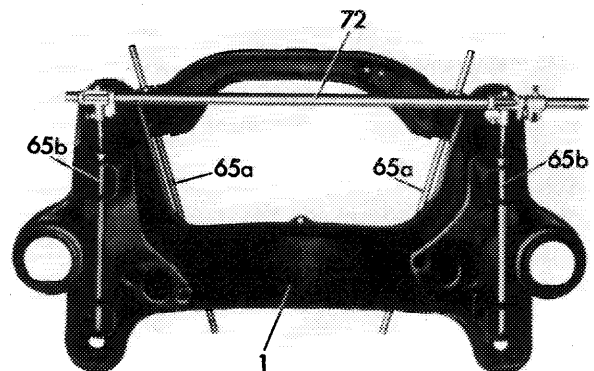
1 Front axle carrier 65a Measuring rods for lower control arm bearing 65b Measuring rods for upper control arm bearing 72 Beam compass
