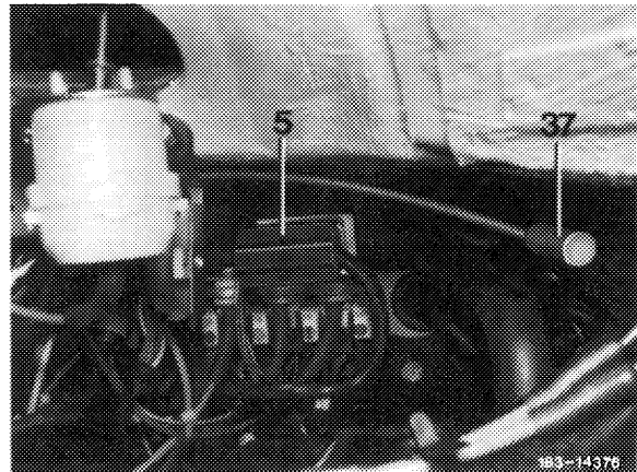
5 10-point plug connection for tester 37 Vacuum connection for tester
