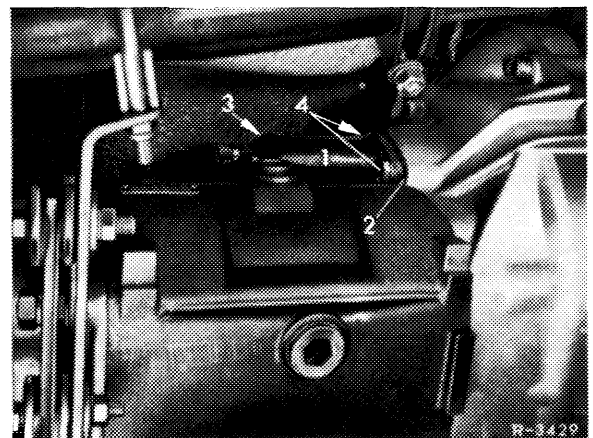
1 Slave cylinder
