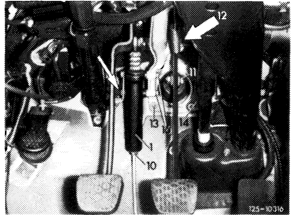
1 Master cylinder
